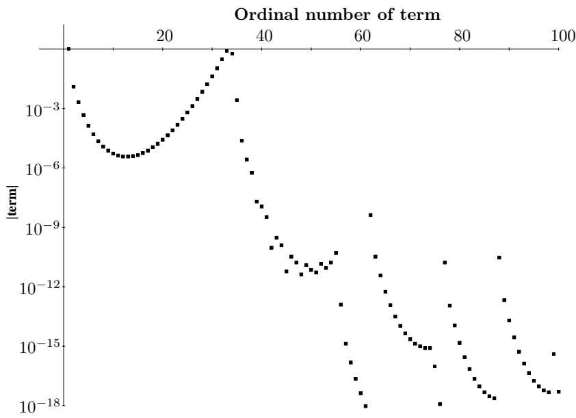
Fig. 10. The terms in (4.53), the level two hyperasymptotic expansion of w_3(z, \eta) . The first (U-shaped) group of terms are the terms in the original asymptotic expansion. The next three groups are the level one re-expansions, and the final four groups are the level two re-expansions.
