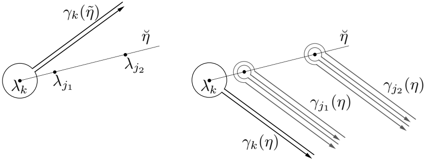
Fig. 7. \gamma_k(\tilde{\eta}) before (left) and after (right) the rotation.
